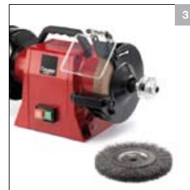
Fixing extension spindle
