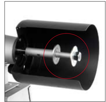
Extension shaft for right-hand side of DS 9200 and DS 9250, distance between flanges 60 mm
